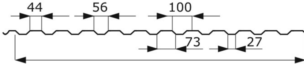
Roof version
