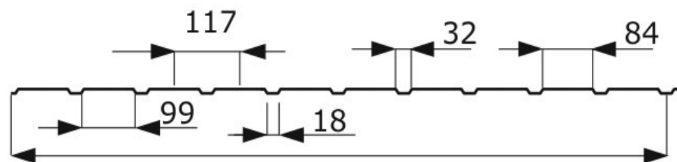
Façade version
