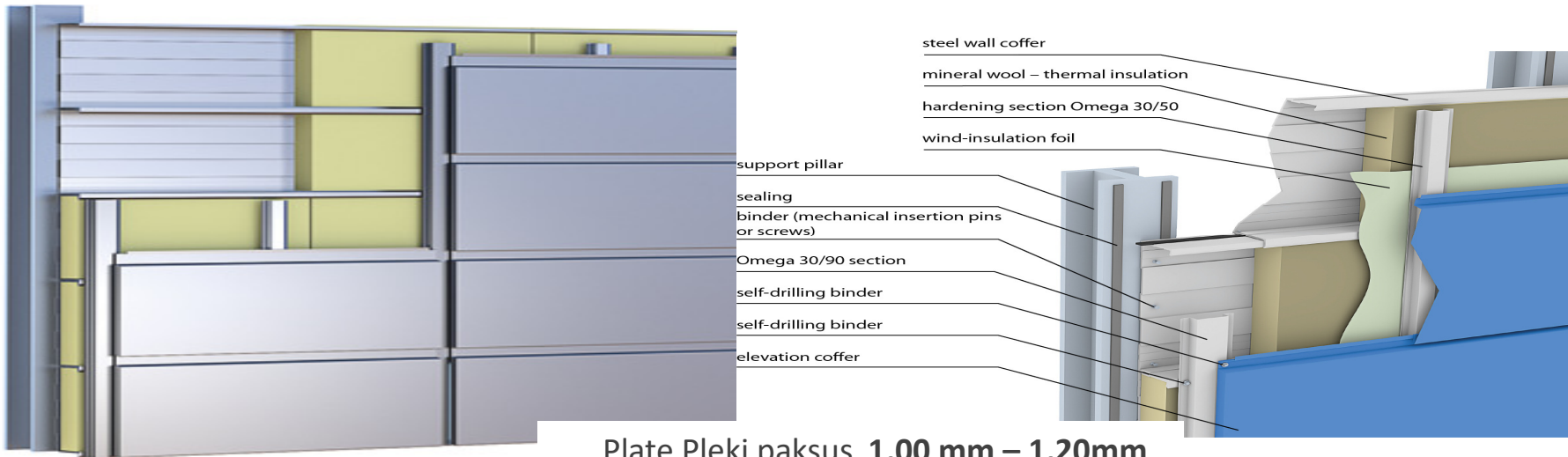
Cross-section - horizontal binding
