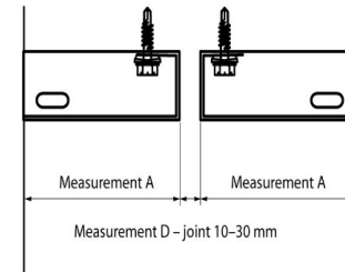
Cross-section - vertical binding
