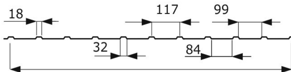
Roof version
