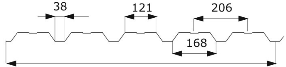
Façade version
