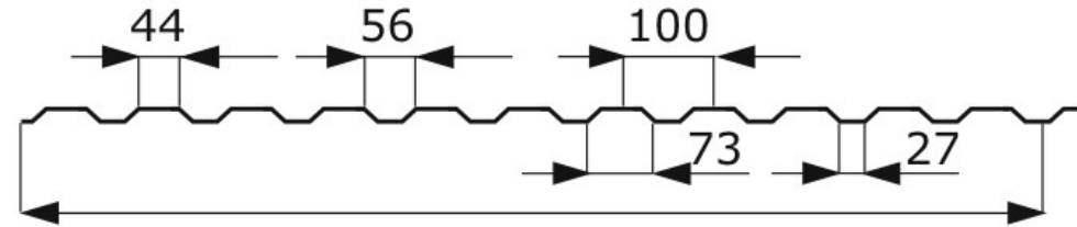
Façade version
