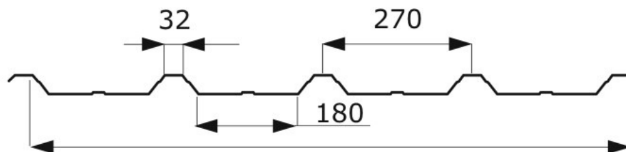
Roof version
