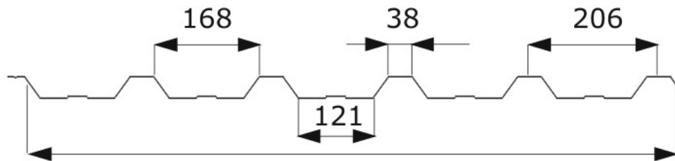
Roof version
